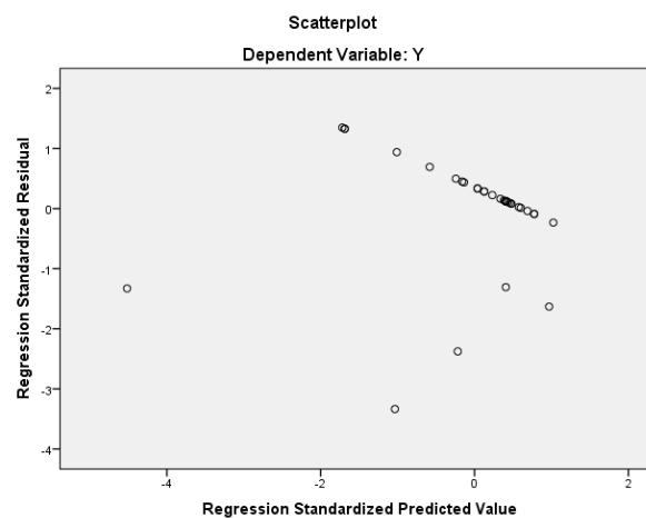
Gambar 2 Scatterplot
