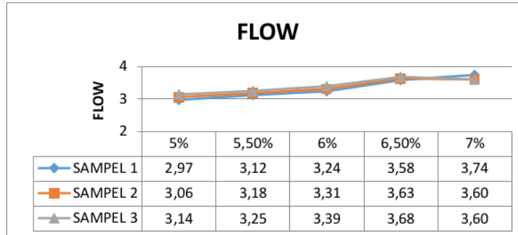
Gambar 5. Nilai Flow.
