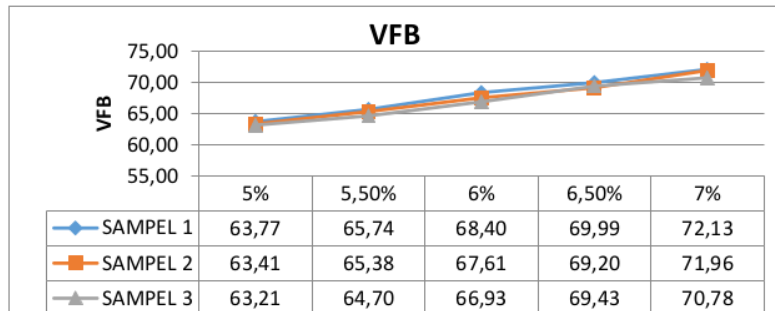
Gambar 3. Nilai VFB.
