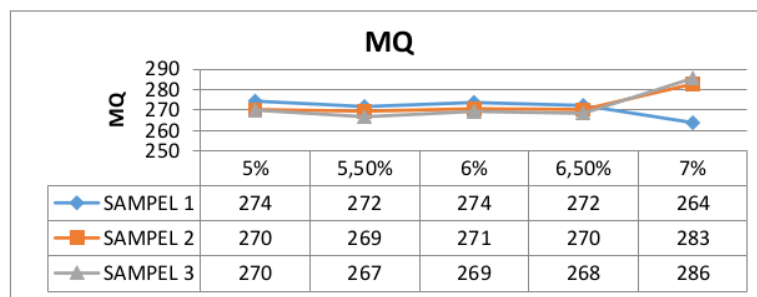
Gambar 6. Nilai MQ.
