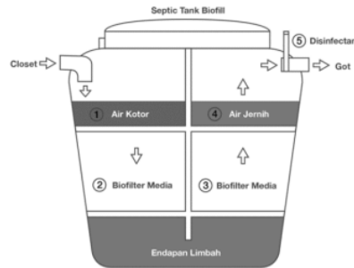
Gambar 6. Biofilter Septic Tank.
