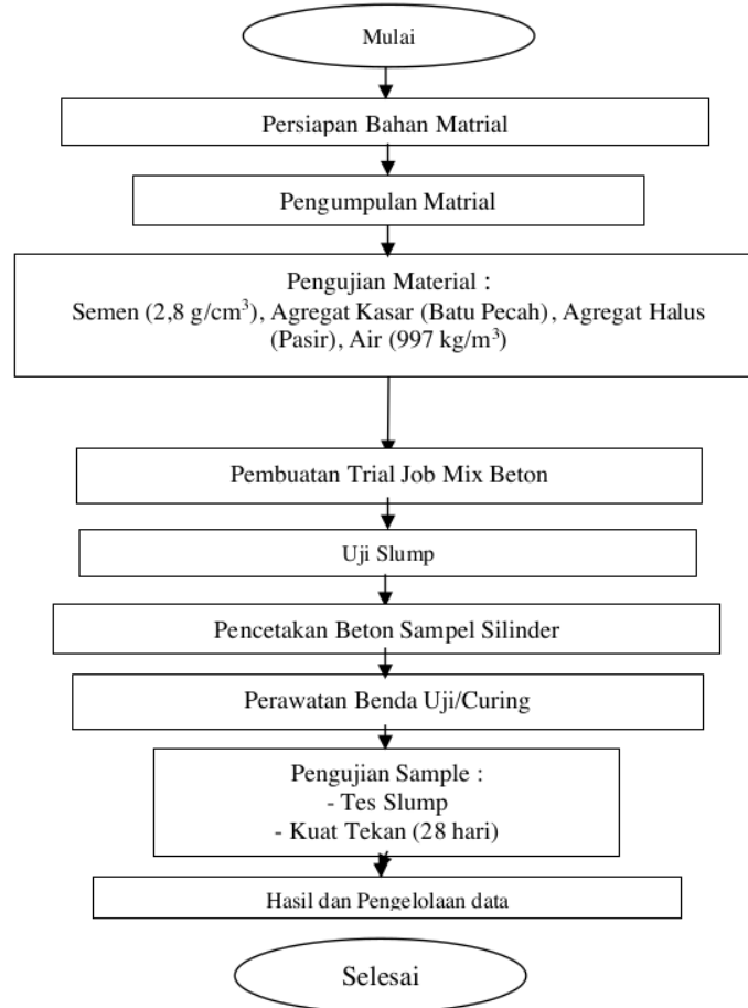
Gambar 3. Flowchart
