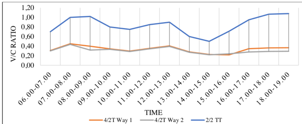
Figure 2. V/C Ratio.
