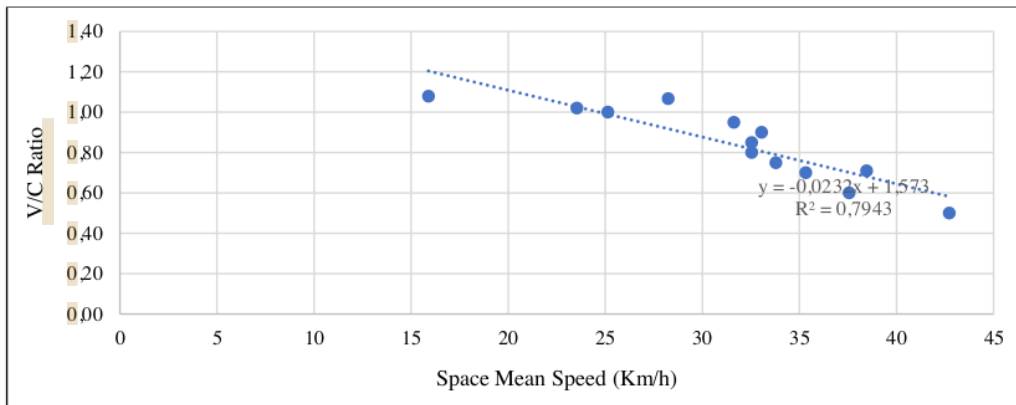
Figure 3. Relationship Between V/C Ratio and SMS.
