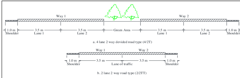
Figure 1. Cross Section Of Piet A. Tallo Street.
