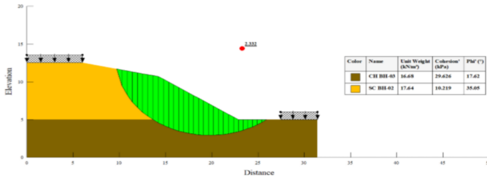
Source : Simulation result for Slope Failure Analysis (Slope/W)
