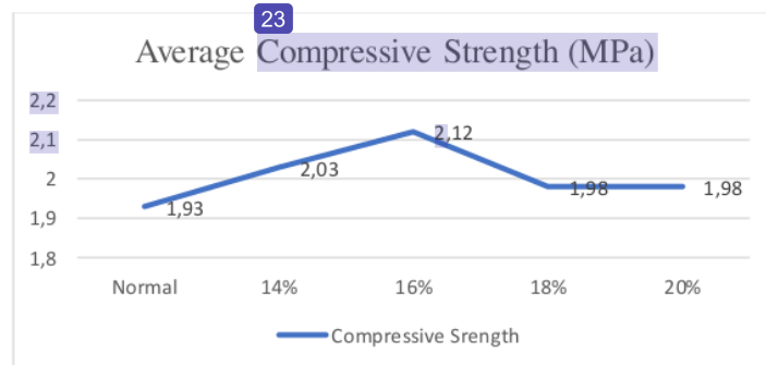
Figure 7. Chart of Average Compressive Strength of Bricks
