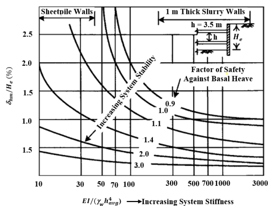
Figure 2. Design Curve Lateral Wall Deformation for Excavation
