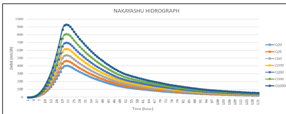
Figure 3. Nakayasu Synthetic Hydrograph
