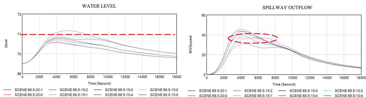
Figure 7. Output Graph of Variable Water Level and Spillway Outflow
