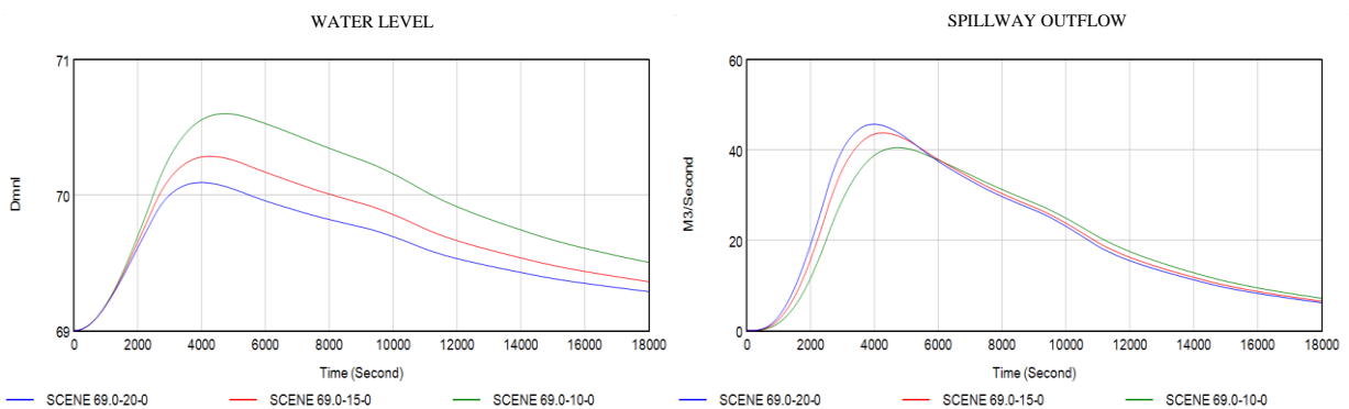
Figure 5. Output Graph of Variable Water Level and Spillway Outflow
