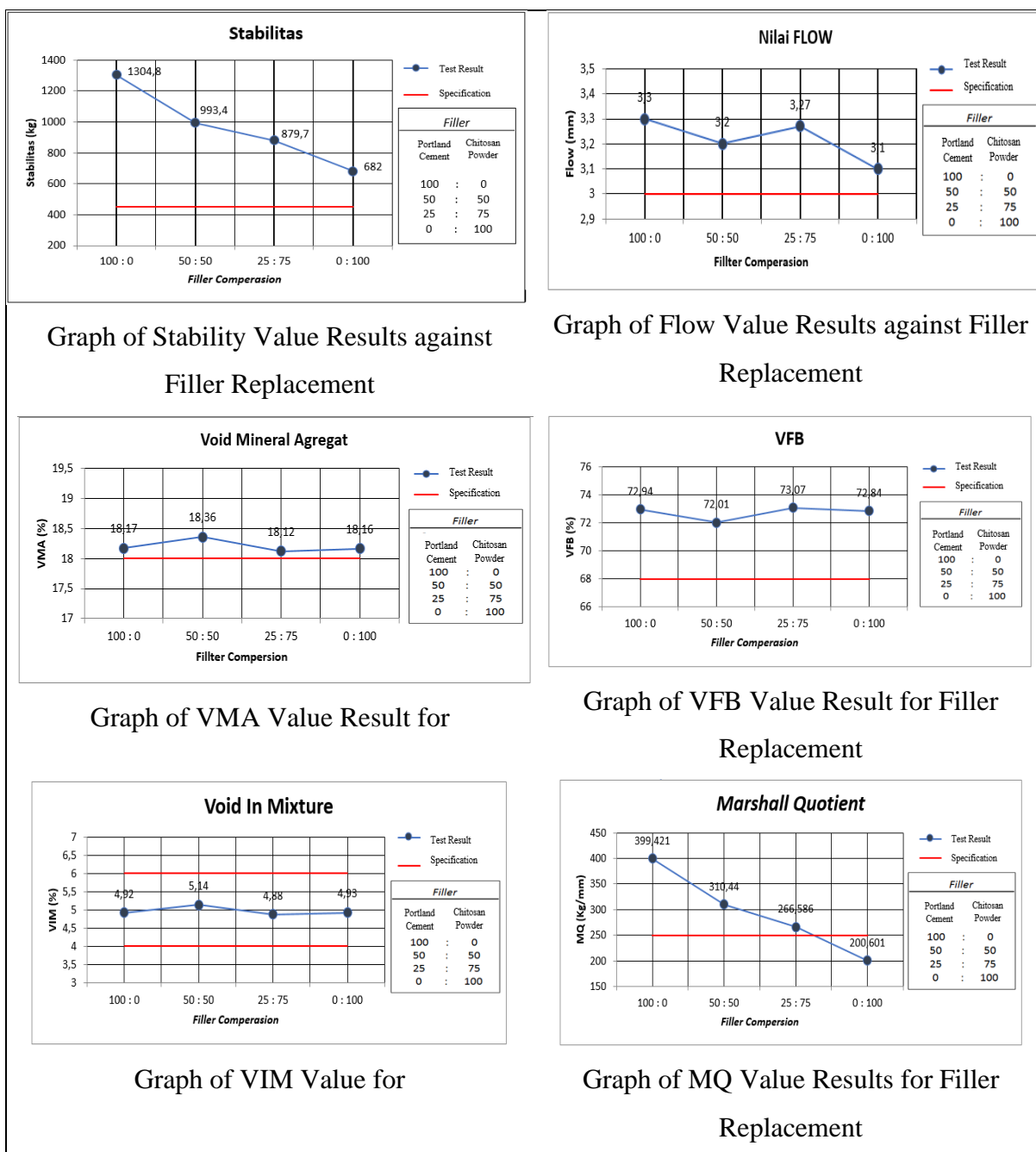
Figure 3. Marshall Test Result
