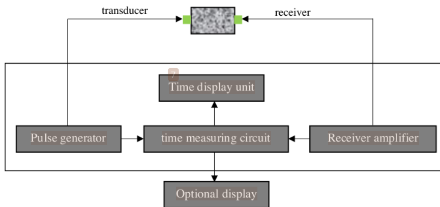
Figure 2. The Mechanism of the UPV Test
