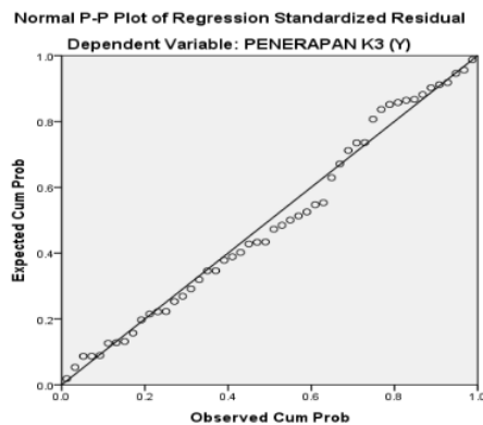
Gambar 1. Grafik Normal Probability Plot.
